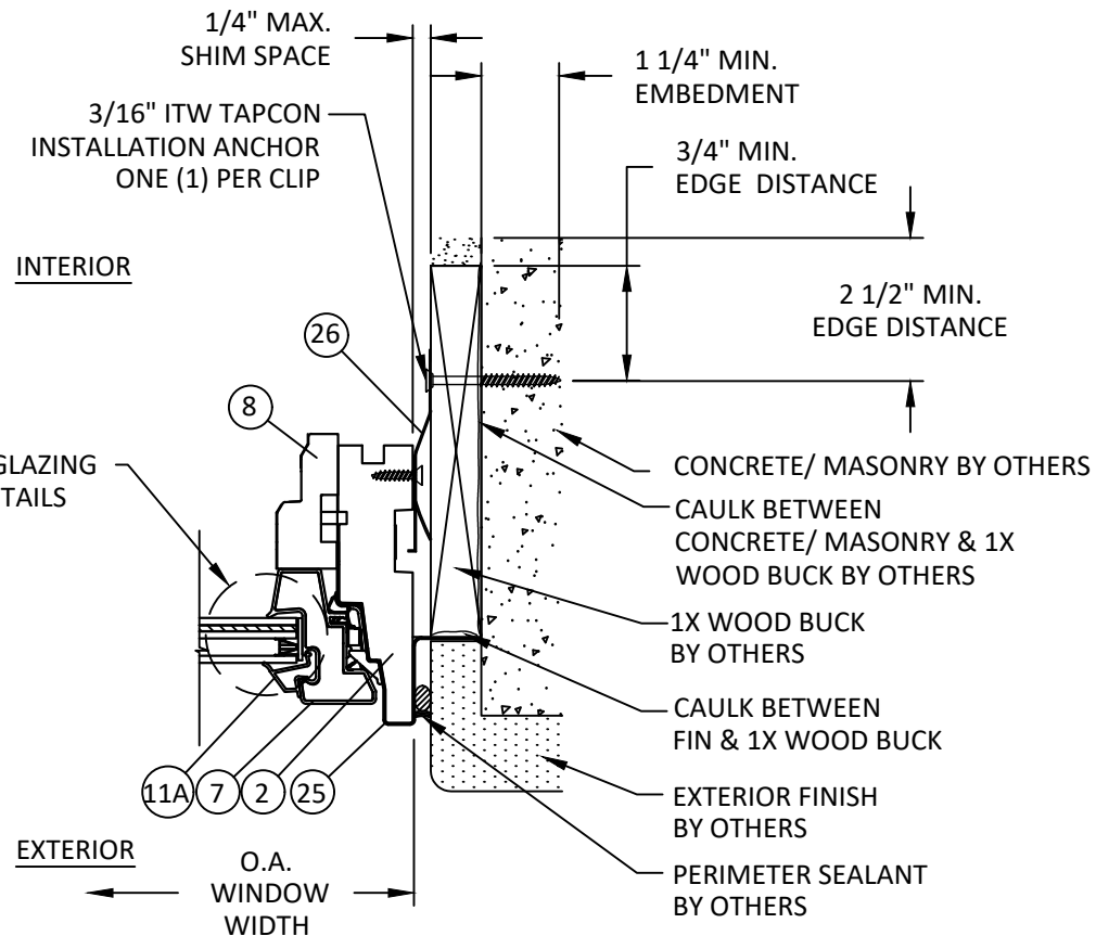
G 5 HORIZONTAL SECTION JAMB - 1X WOOD/CONCRETE/MASONRY INSTALLATION CLIP
