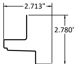
25A FRAME HEAD/SILL CLADDING PVC
