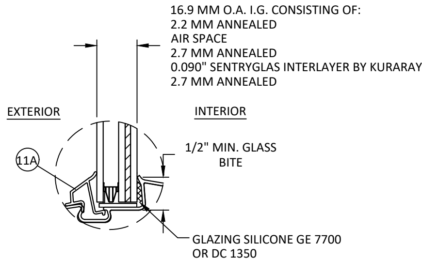
GLAZING DETAIL 1
