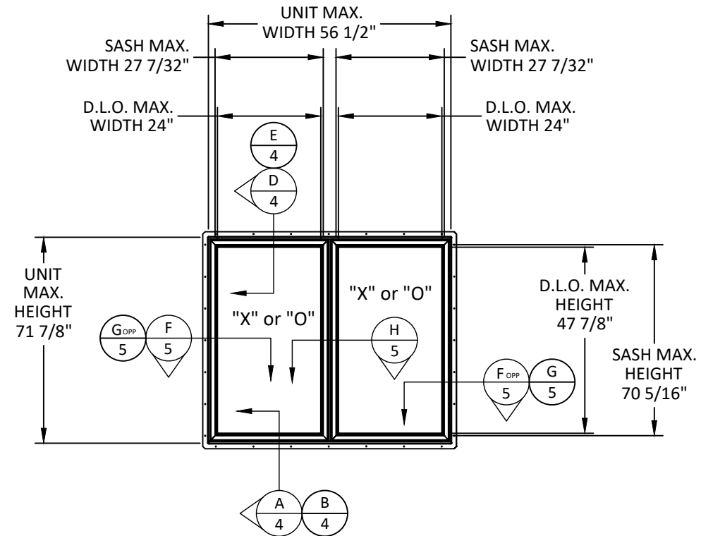
ELEVATION CW26
