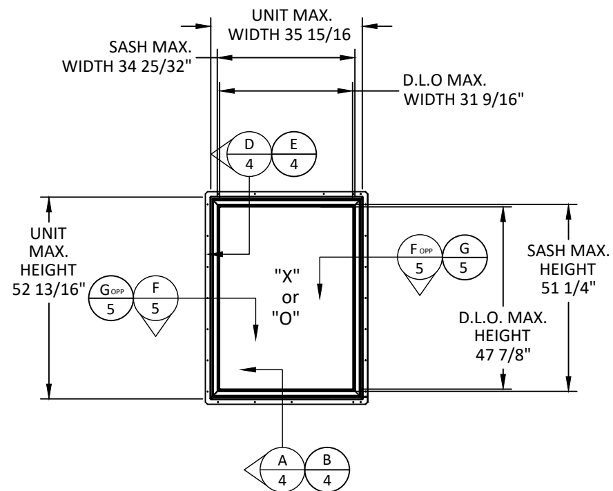
ELEVATION CXW145
