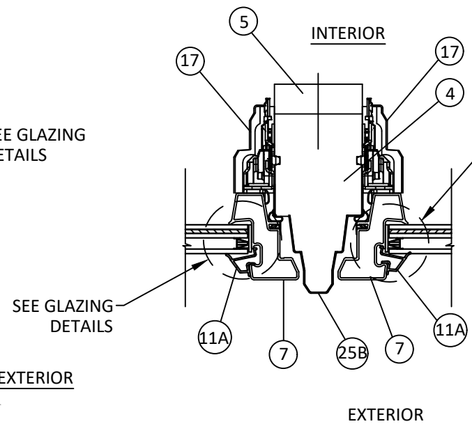
H 5 HORIZONTAL SECTION INTEGRAL MULLION POST
