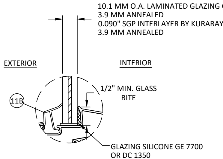
GLAZING DETAIL 2
