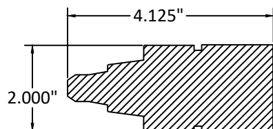
6 SASH RAIL/STILE CLAD. PVC
