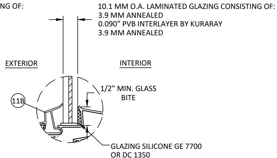
GLAZING DETAIL 3
