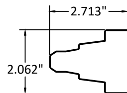
7 SASH RAIL/STILE WOOD
