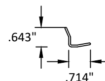
28 EXTERIOR SNUGGER ALUMINUM
