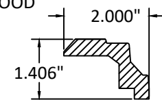
25 FR. SIDE CLADDING PVC
