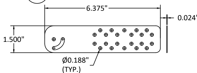
27 INSTALLATION CLIP 304 SS
