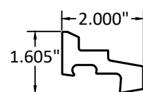
11 GLAZING BEAD - I.G. PVC
