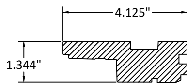
3 EXTENSION JAMB WOOD
